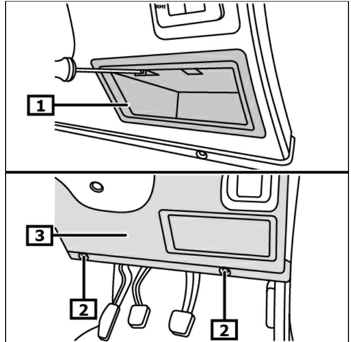
1 Vide-poches 2 Vis 3 Cache
