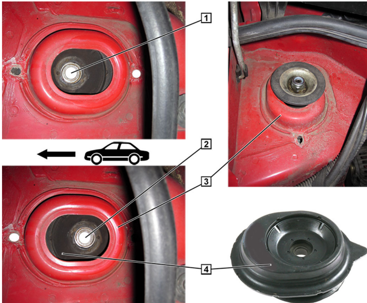
Fig. 1: Suspension strut mount in different installation positions
