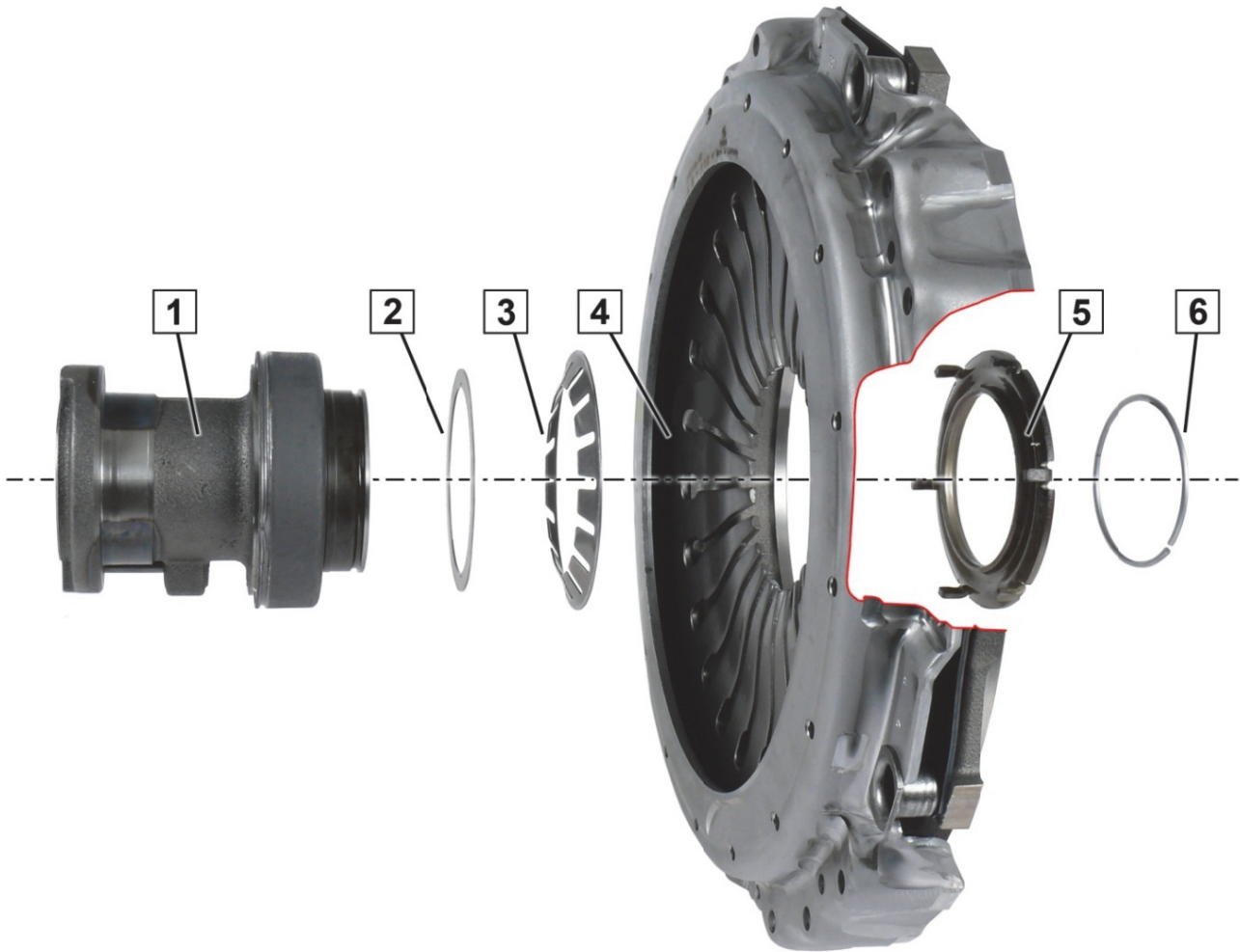
Fig. 1: Clutch release with fixed connection. Assembly sequence and component alignment.
