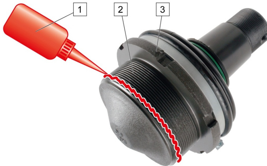
Fig. 1: Supporting joint, thread securing agent
